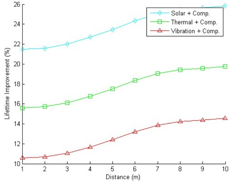
Figure 4.4.17. Lifetime improvement with joint utilization of compression and energy harvesting approaches wrt. distance for Telos
