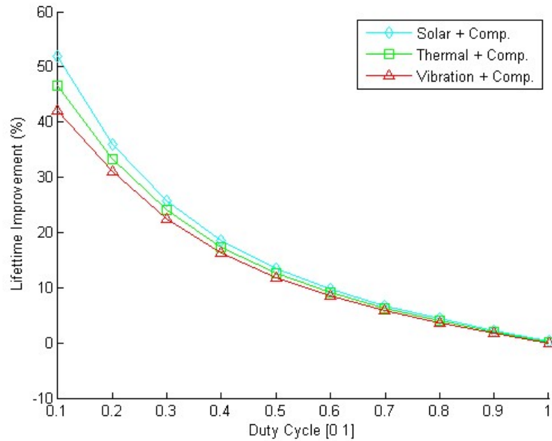
Figure 4.4.16. Lifetime improvement with joint utilization of compression and energy harvesting approaches wrt. duty cycle for Mica2
